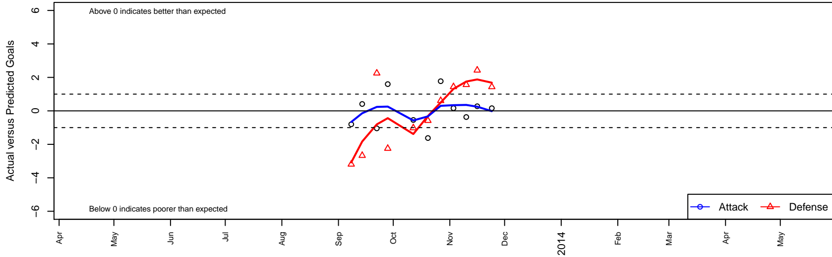
FC Impact Blue B96 Dots are actual minus expected GF (blue circles) and GA (red triangles). Blue line is smoothed change in attack strength. Red is smoothed change in defense strength.
